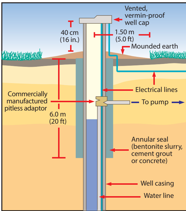
Cross-sectional illustration of a drilled well with a pitless adaptor. Reproduced with permission from the Ontario Ministry of Agriculture, Food and Rural Affairs, 2016.
