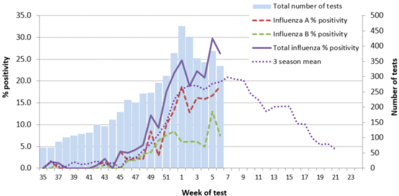
Figure 3: Percent and number of nasopharyngeal specimens that tested positive for influenza in Ottawa, 2019-2020 season to week 6, by influenza type
