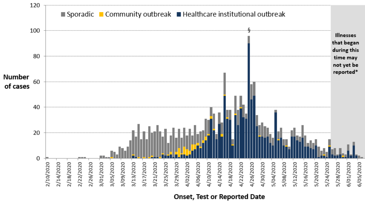
Figure 3. Epidemiological curve of Ottawa residents with confirmed COVID-19, by the EARLIEST of onset, test and reported date, by outbreak association† (n=2,006)
