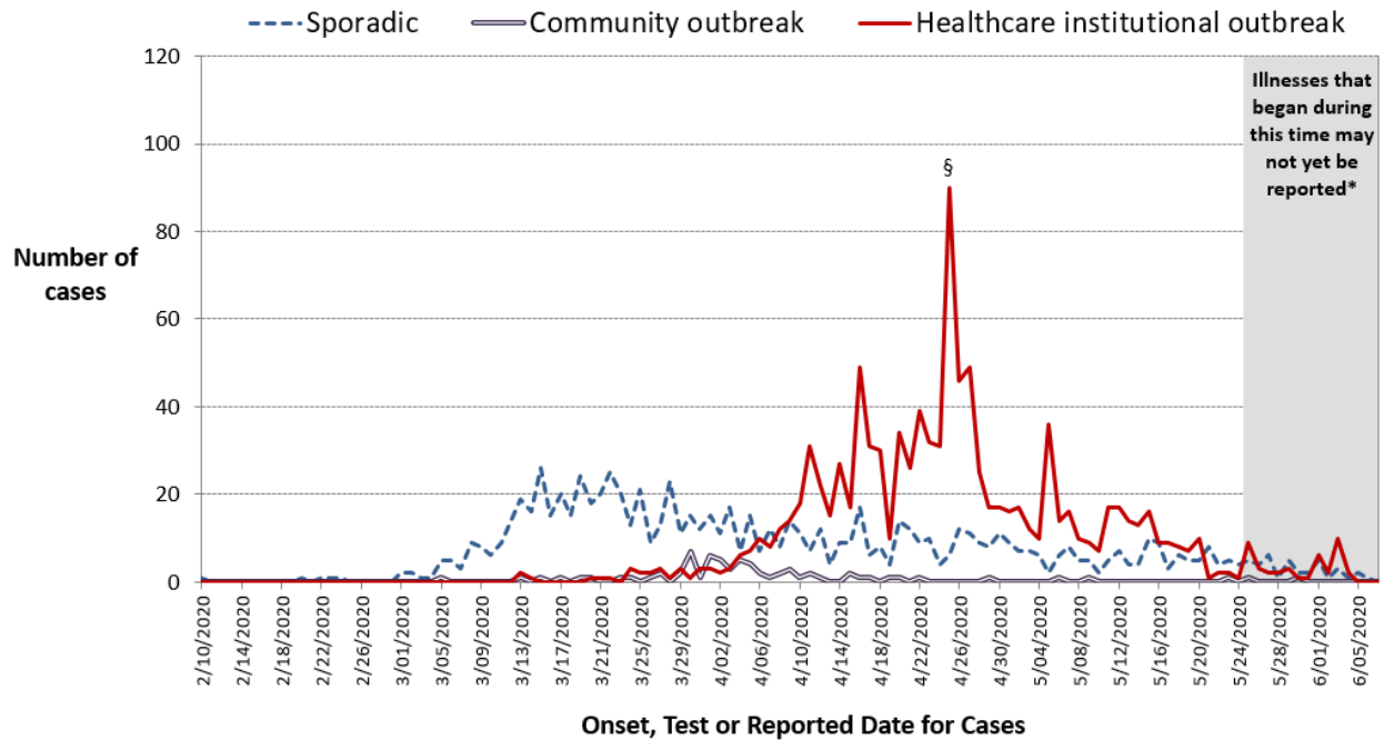
Figure 2. Epidemiological curve of Ottawa residents with confirmed COVID-19, by the EARLIEST of onset, test, and reported date, by outbreak association† (n=2,006)
